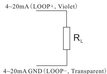
Figure 6-4. 4~20mA External Connection
