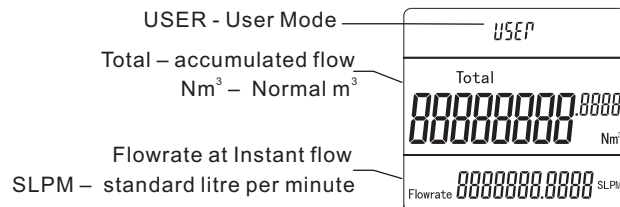
Figure 6-3a. Normal Display
